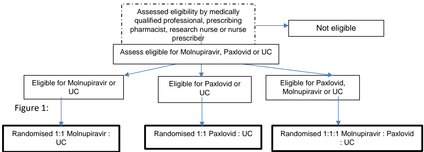
Example of eligibility flow for randomisation when adding Paxlovid as a new intervention.
